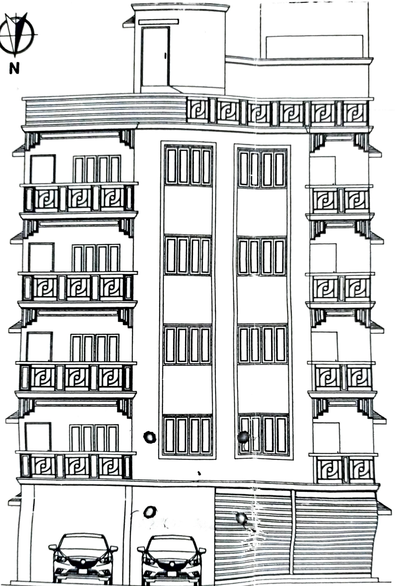
FRONT ELEVATION (BLOCK 1) (SCALE - 1:100)
